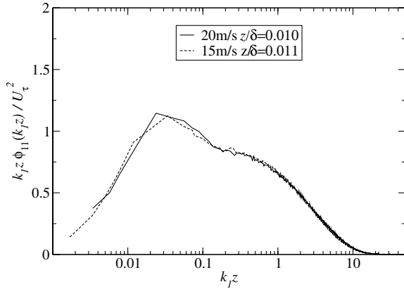
FIG. 4. Streamwise spectra in inner scaling for two tunnel velocities and virtually the same z/\delta . 20 m/s: z^+ = 150 ; 15 m/s: z^+ = 118 . Note that only inner scaling is shown. The collapse would be the same in outer scaling since the z/\delta is closely matched.
