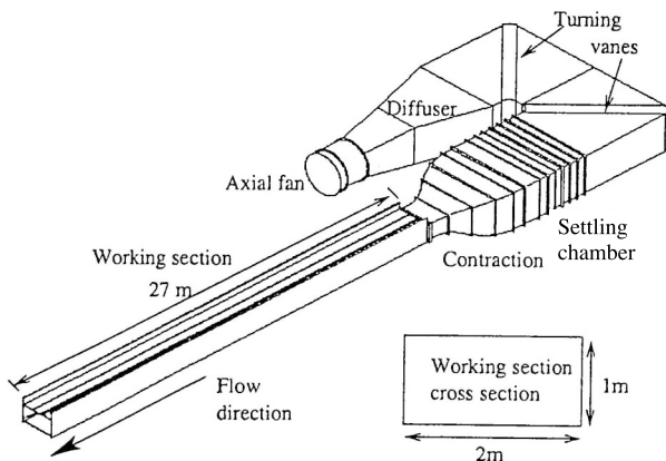
FIG. 1. Schematic of wind tunnel used in this study.
