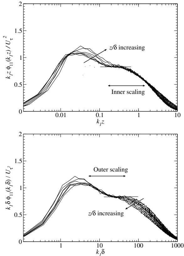
FIG. 2. Streamwise spectra in inner scaling (upper plot) and outer scaling (lower plot). Wave number calculated using U_c equal to local mean velocity at each wall-normal position. Levels shown: z/\delta = 0.0070, 0.0077, 0.0084, 0.0092, 0.0205, 0.0123, 0.0140 . The lowest level corresponds to z^+ = 100 .
