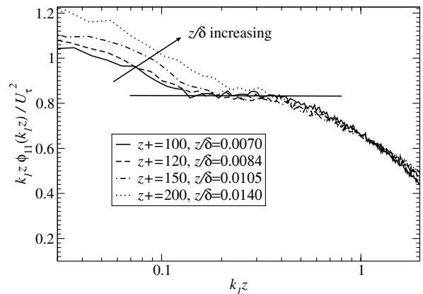
FIG. 3. Close-up of the k_1^{-1} region of spectra in premultiplied form. Wave number calculated using U_c = \bar{U} . Inner scaling.
