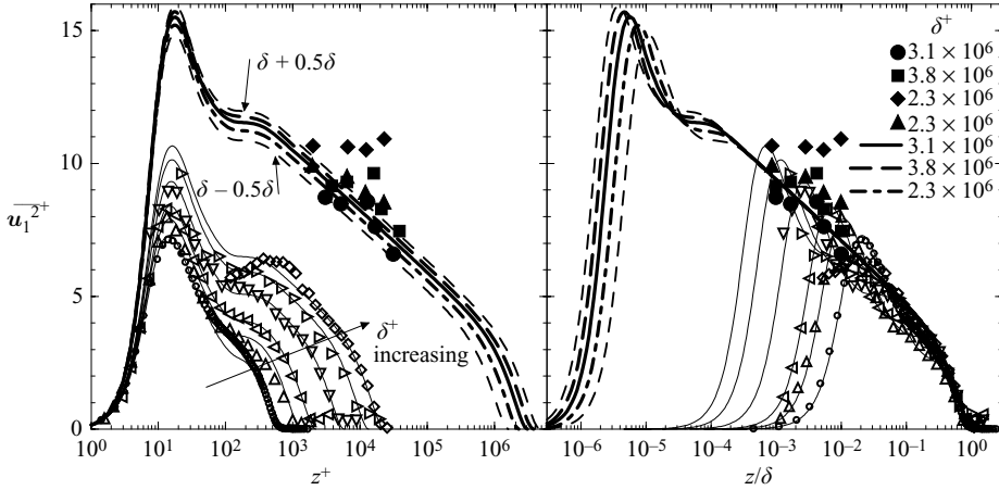
FIGURE 4. Streamwise turbulence intensities. Solid symbols are atmospheric data. Open symbols are laboratory data; \delta^+ = 689 ( \circ )–Spalart (1988); 1335 ( \Delta ), 2217 ( \nabla ), 5813 ( \triangledown ), 13 490 ( \triangleright )–DeGraaff & Eaton (2000); 23 013 ( \diamond )–Fernholz et al. (1995). Solid, dashed and dot-dashed lines are smooth-wall similarity formulations (equation (2.1)) that are also valid for rough walls in the outer region. Lighter dashed lines are similarity formulation for \delta^+ = 3.1 \times 10^6 if boundary-layer thickness is 50 % larger or smaller.
