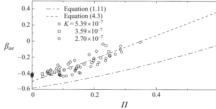
FIGURE 11. Experimental data for \beta_{ae} from current study along with curve fits.
